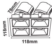
Dimension ( mm )
